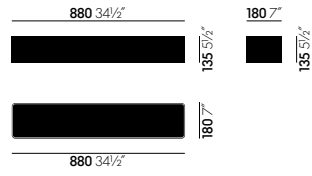
Caisson suspendu
